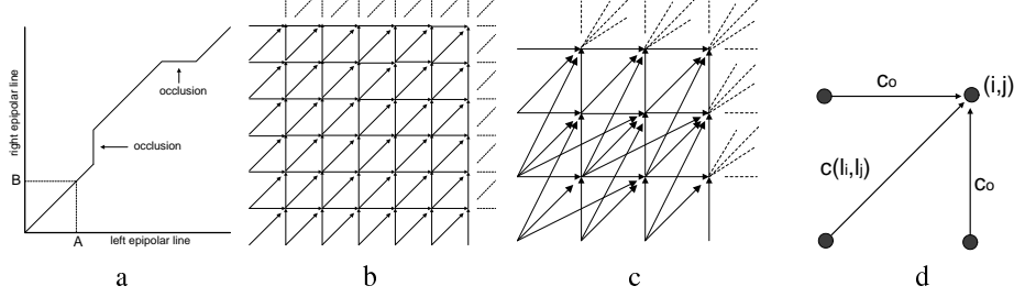
Figure 2: Dense epipolar matching. (a) the path defines a matching between the two epipolar lines, e.g. point A is matched to point B. Horizontal and vertical arcs represent occlusions. (b) the connectivity of the graph of the Cox et al method, each vertex represents a putative matching of a left and right pixel and has three input arcs and three output allowing horizontal, vertical and diagonal moves. (c) the connectivity of the Geiger et al method, here more complex movements can be made. (d) The input to a node for the maximum likelihood model. Horizontal and vertical moves mean that a point is unmatched and are assigned cost c_0 , the diagonal move means that the i th left pixel is matched to the j th right pixel with cost c(l_i, r_j)
